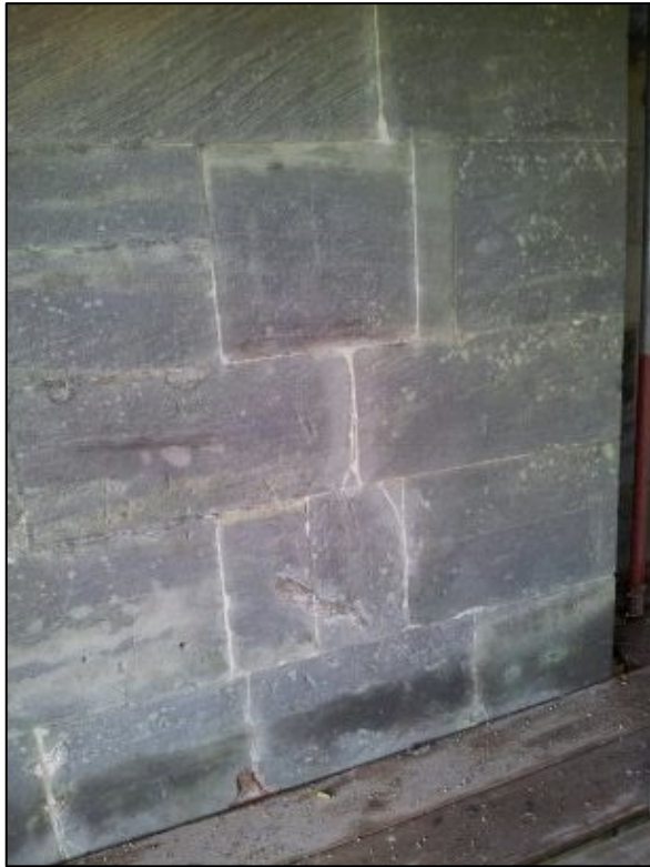
The ashlar blocks are beautifully dressed and fitted with very tight joints, making repointing a painstaking process.
